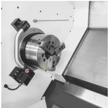
RENISHAW brand tool setting probe
